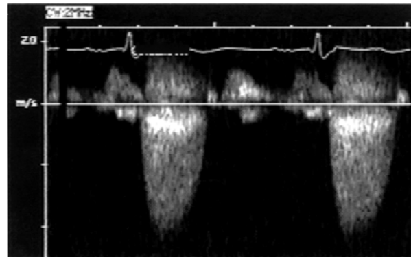
Figure 2 CW Doppler recording of velocity through aortic valve in patient with AS. Transducer position is at apex; thus systolic velocities are displayed below baseline. In diastole, positive mitral inflow velocities can be seen as inflow moves toward transducer. Note wide spectral dispersion of velocities during systole and diastole indicating that Doppler beam is detecting all flow velocities encountered along its course.
